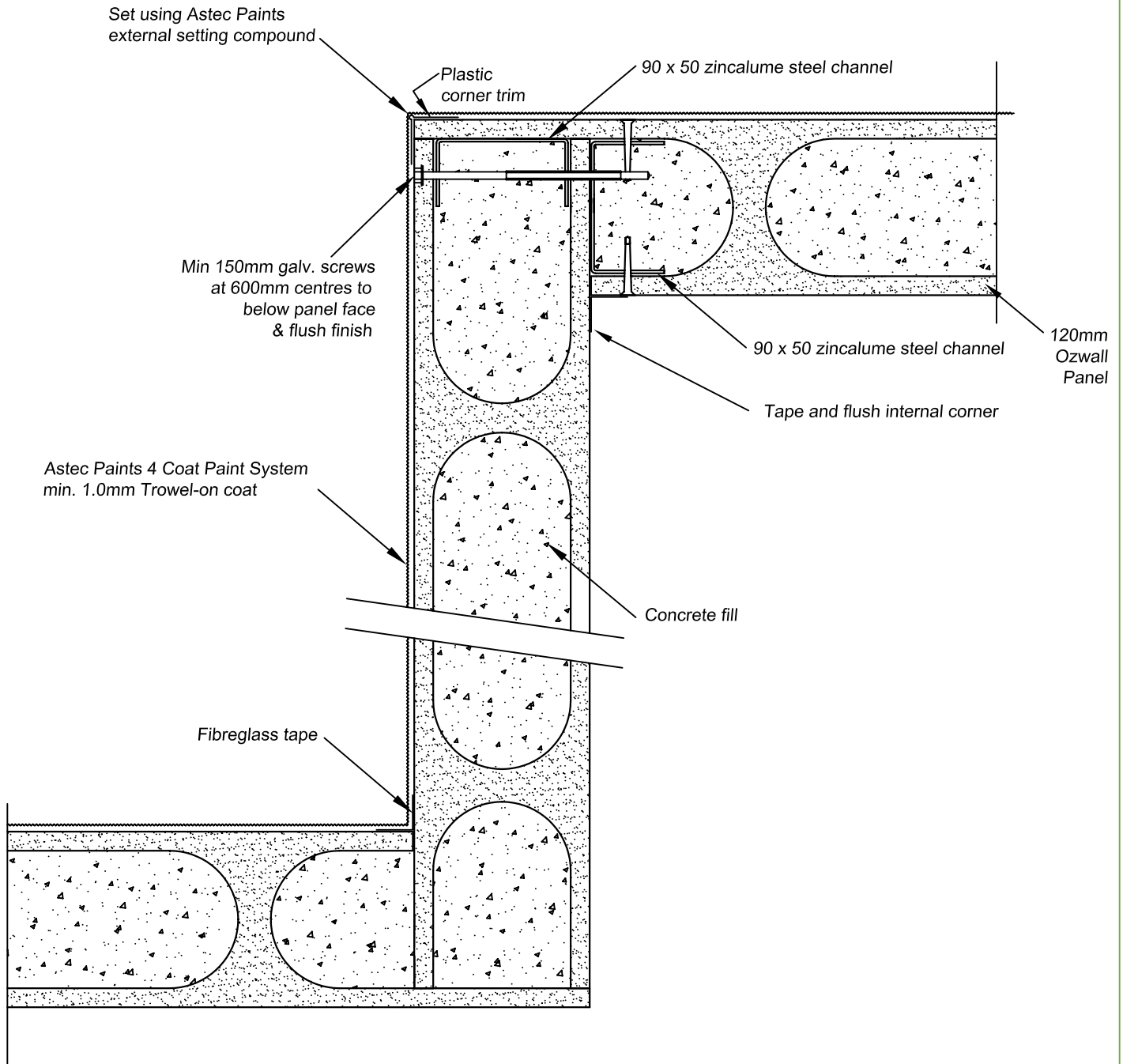
STANDARD CORNER JUNCTION (plan view)
