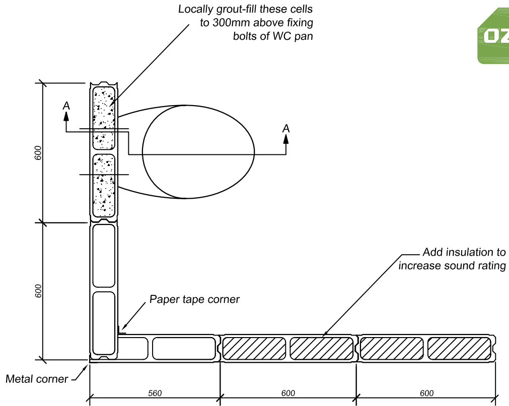
TYPICAL PANEL LAYOUT (plan view)
